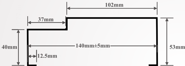
Single Collar Door Frame
